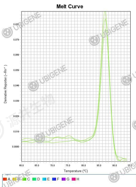
ASGR1 Stable Expression Cell Line (293T)+hASGR1 - 1 melt curve
