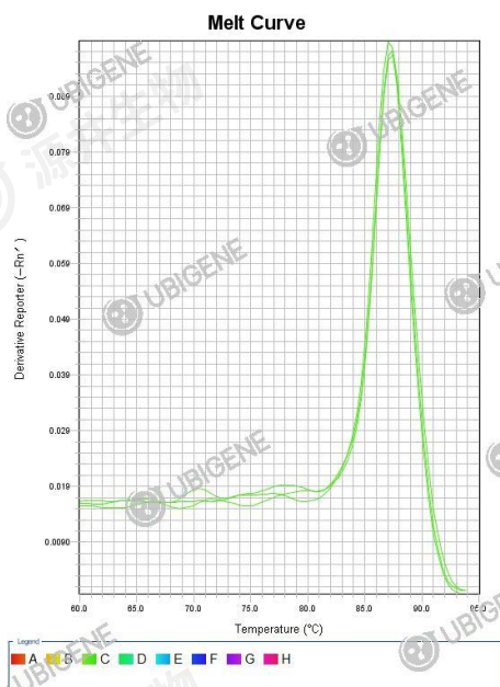
293T_Ctrl(Puro)+hASGR1 -1 melt curve
