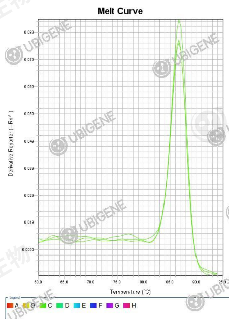
ASGR1 Stable Expression Cell Line (293T)+ \beta -h_actin melt curve
