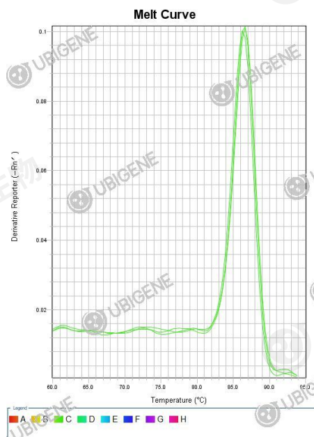
293T_Ctrl(Puro)+ \beta -h_actin melt curve
